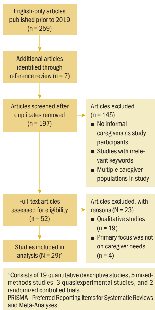
FIGURE 1. PRISMA Flowchart
